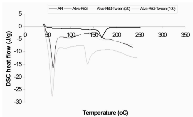
Figure 5. DSC curve for atorvastatin-poly ethylene glycol-tween 80 combination.
